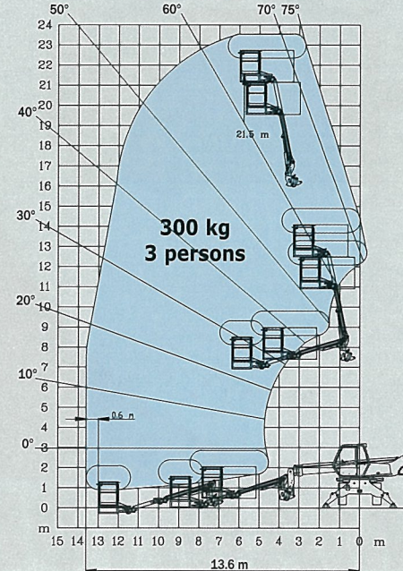
ROTATION ON STABILISERS WITH AERIAL JIB PLATFORM
