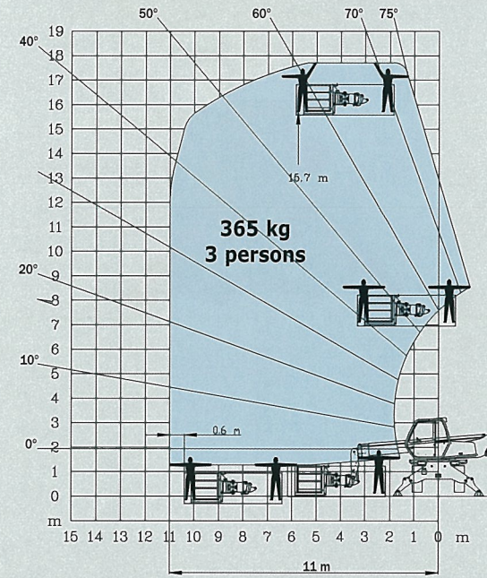
ROTATION ON STABILISERS WITH AERIAL JIB PLATFORM
