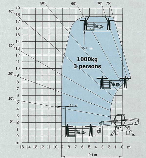
ROTATION ON STABILISERS WITH 1000 KG PLATFORM 2,25/4 m
