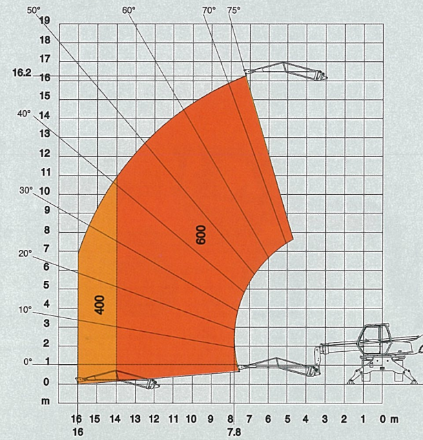
ROTATION ON STABILISERS WITH EXTENSIBLE PLATFORM 2,25/4 m
