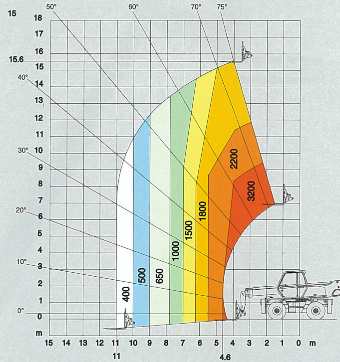
ROTATION ON STABILISERS WITH 3T WINCH
