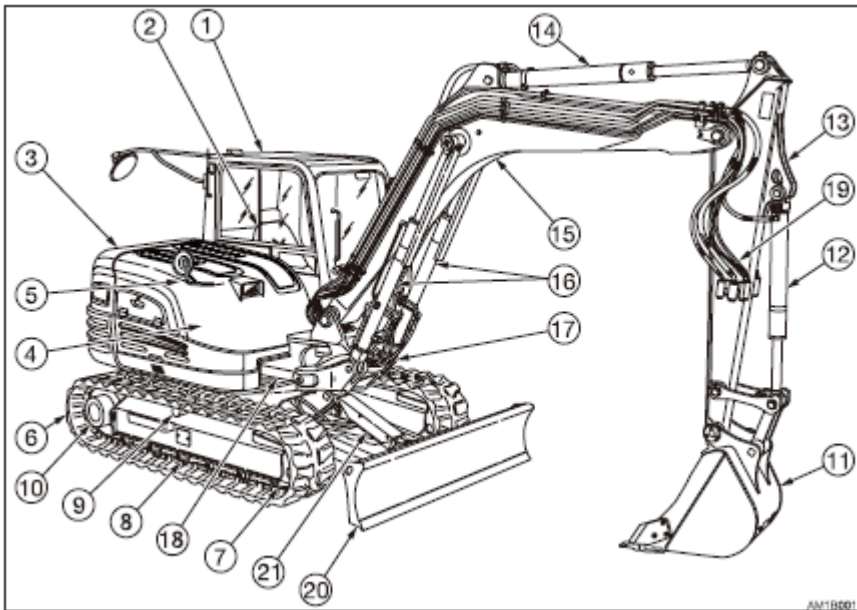
2-Piece boom
